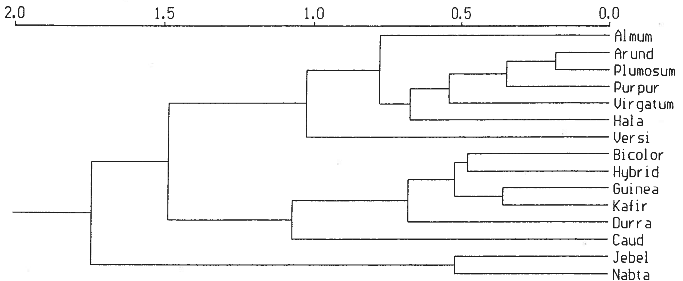
Fig. 4. Phenogram based on full data set of cultivated, wild, and sorghum samples from Nabta Playa and Jebel et Tomat
